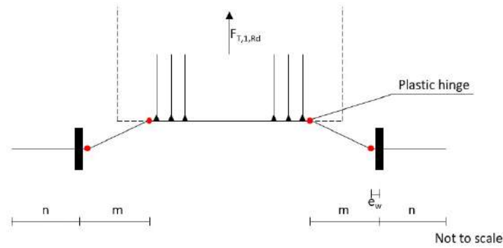
Figure E.20: Mode 1: Complete yielding of the flange
