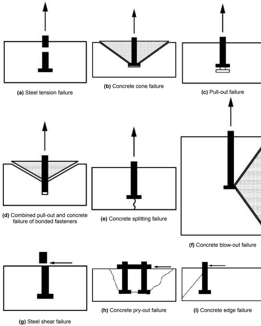
Figure 5.4: Failure mechanisms of anchor bolt [49]
