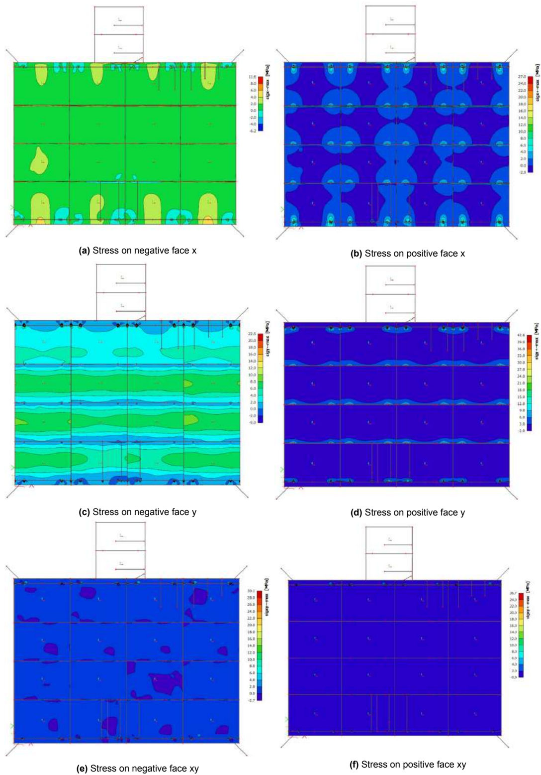
Figure 4.11: Extreme positive stress in faces of reusable jetty deck
