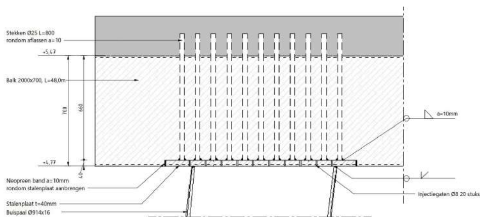
Figure C.3: Detail of fixed pile to beam connection [61]
