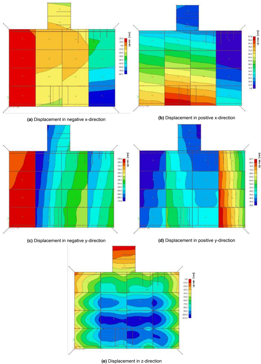
Figure F.4: Displacement of the simple solution using the piles needed for construction
