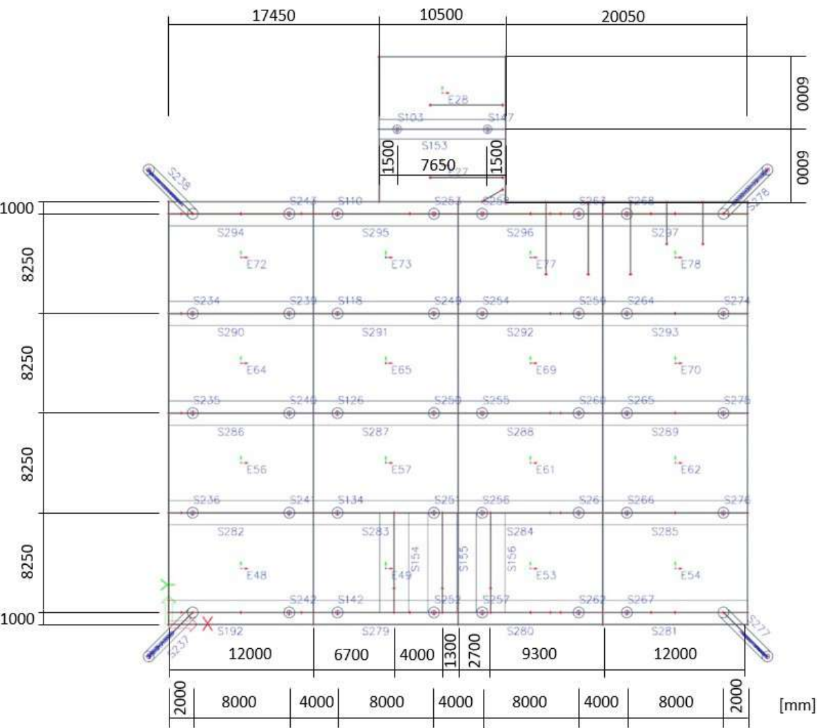
Figure D.5: Layout of reference jetty model
