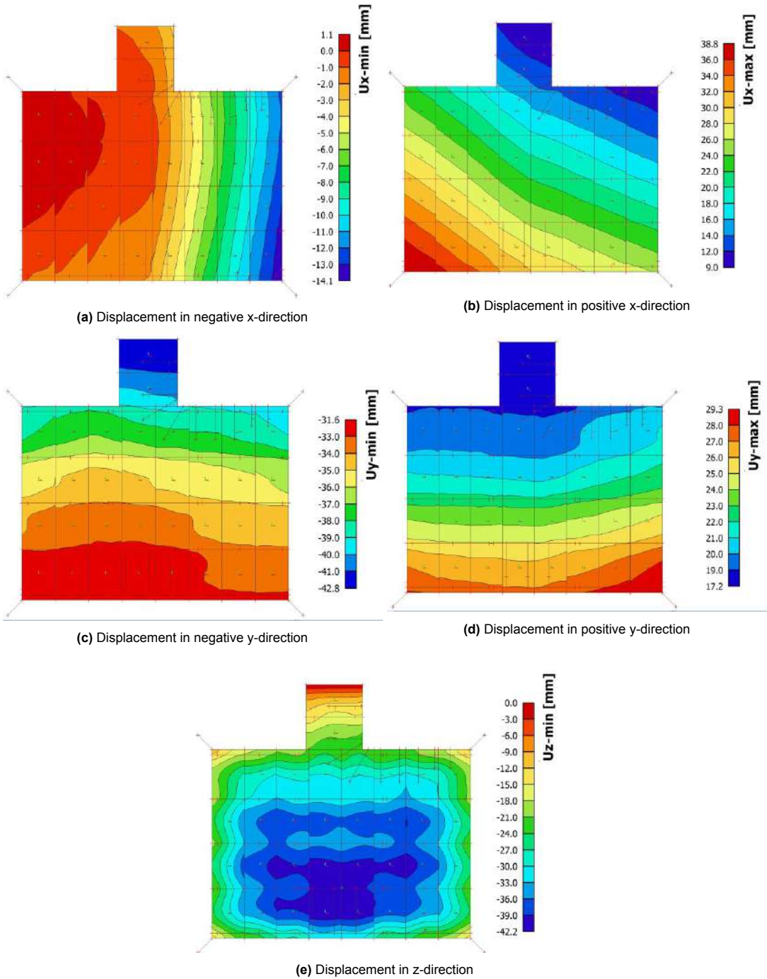
Figure E.6: Displacement of no deck plate to deck plate and shear rib plate to rib plate connection variant 1
