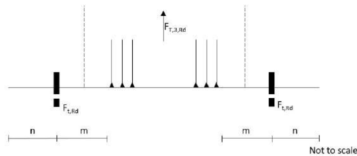
Figure E.22: Mode 3: Bolt failure
