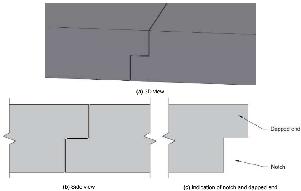
Figure 5.1: Shear rib plate to rib plate connection
