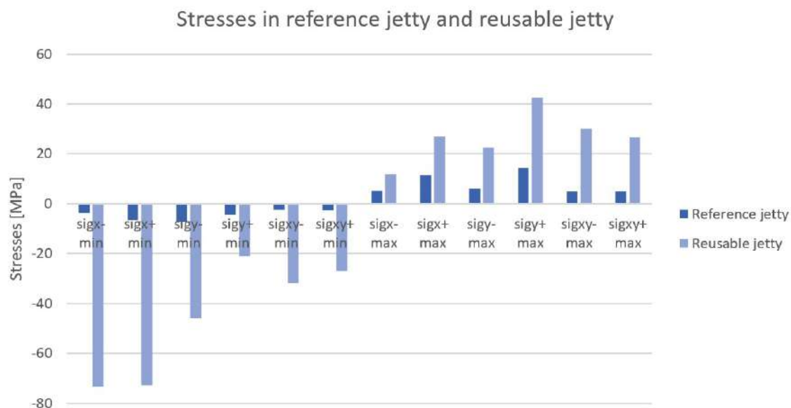
Figure 4.12: Stresses in reference jetty and reusable jetty
