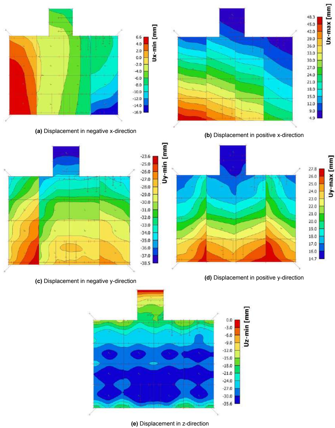
Figure F.3: Displacement of no plate-part to plate-part and shear rib-part to rib-part connection variant 3
