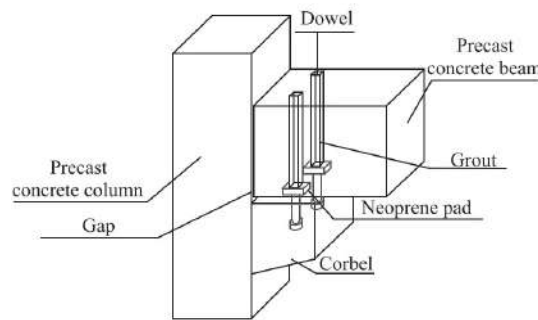
Figure 2.1: Dowel concrete connection [21]
