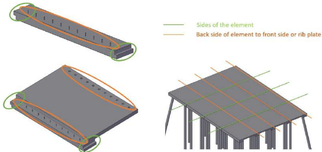
Figure 4.4: Connection types in variant 3
