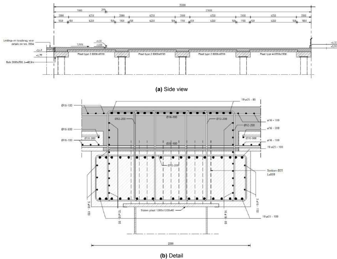
Figure C.4: Overview of rib plate to deck plate connections [61]
