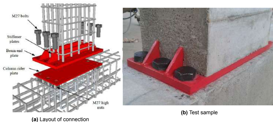
Figure 2.3: Successfully tested dry column to beam connection with rider plate [13]
