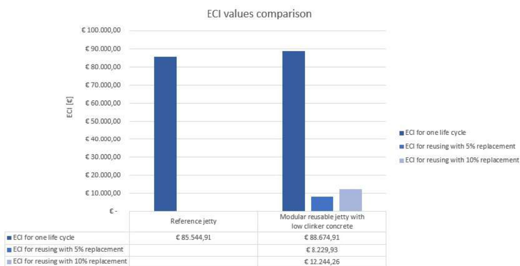
Figure 7.4: Overview of ECI for energy transition
