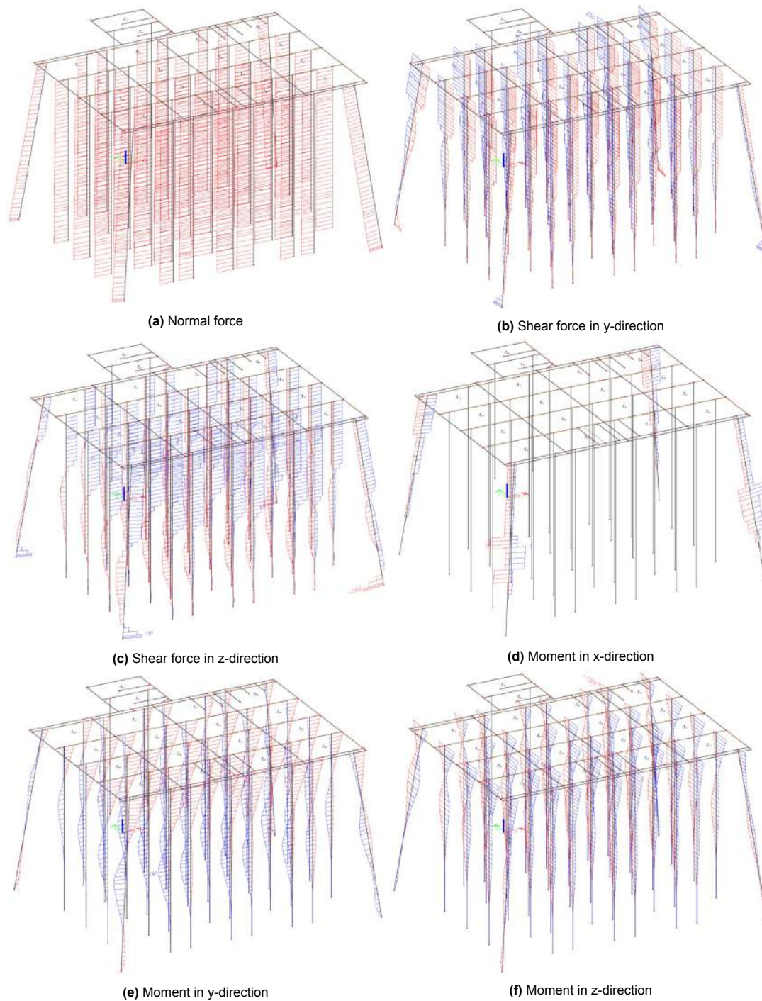
Figure 4.8: Internal forces in piles of reusable jetty
