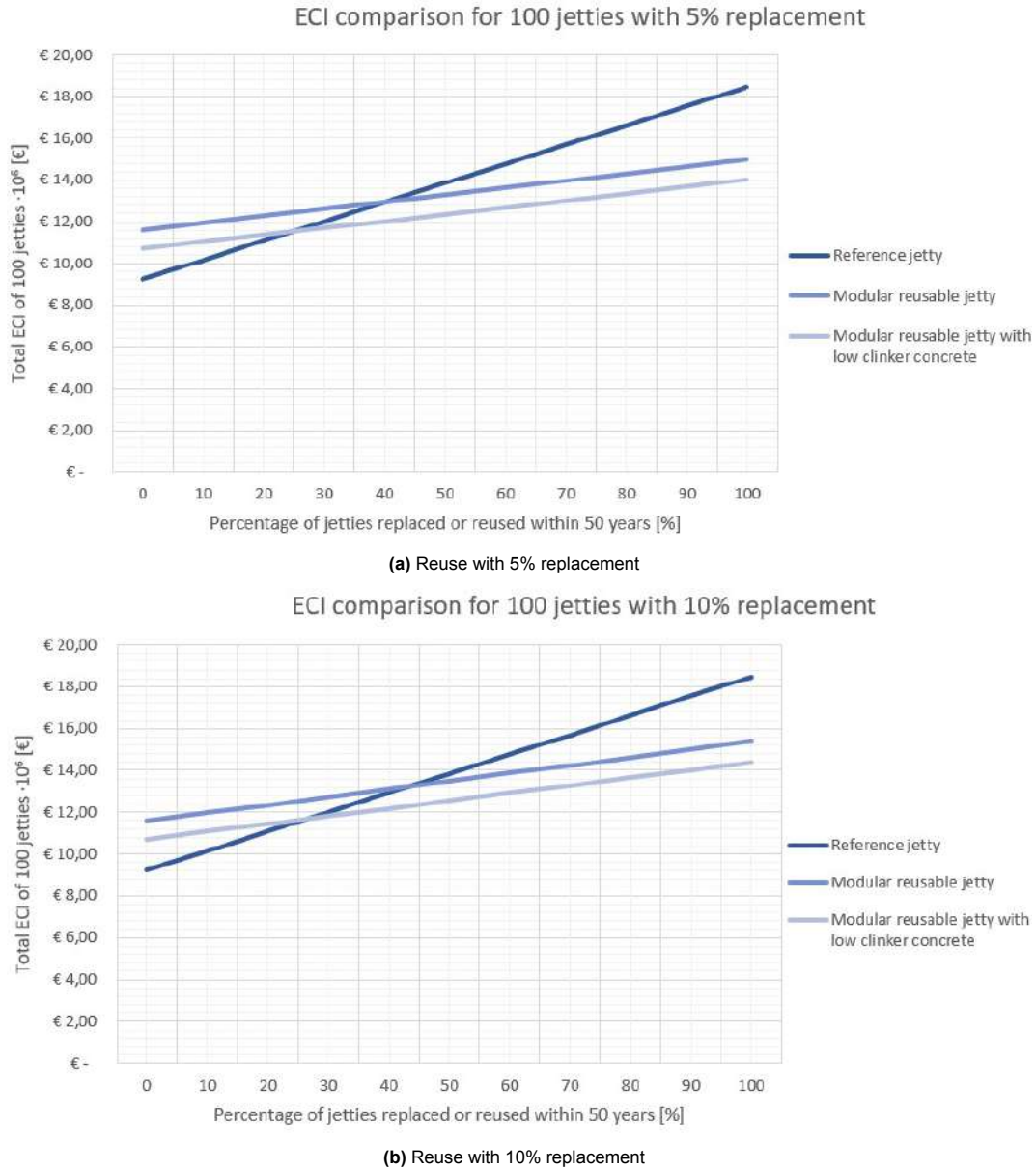
Figure 7.3: ECI comparison for one time reuse of 100 jetties
