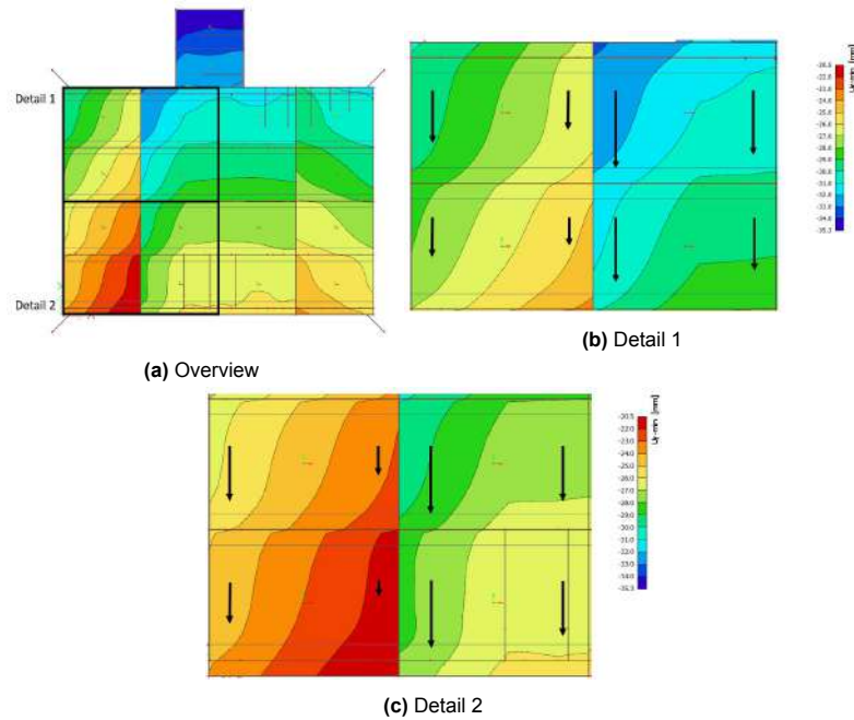
Figure 4.15: Displacement in negative y-direction of reusable jetty deck
