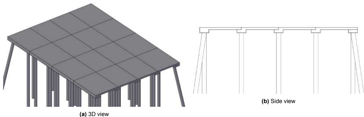
Figure 4.2: Layout of variant 3: Roof tile concept
