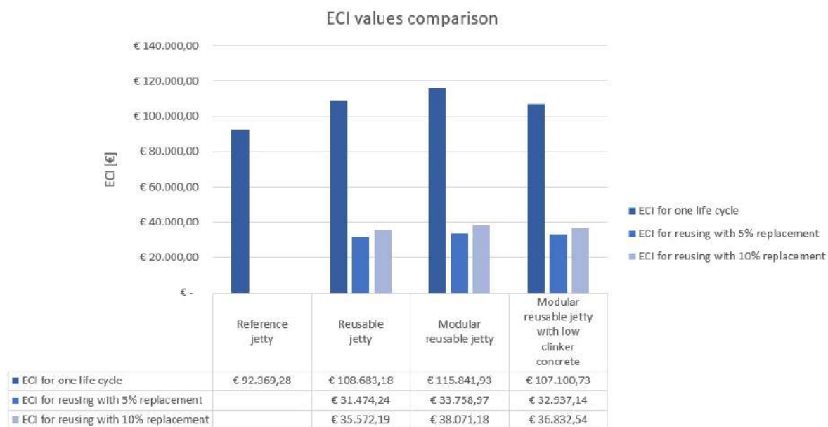
Figure 7.1: Overview of ECI for all variants
