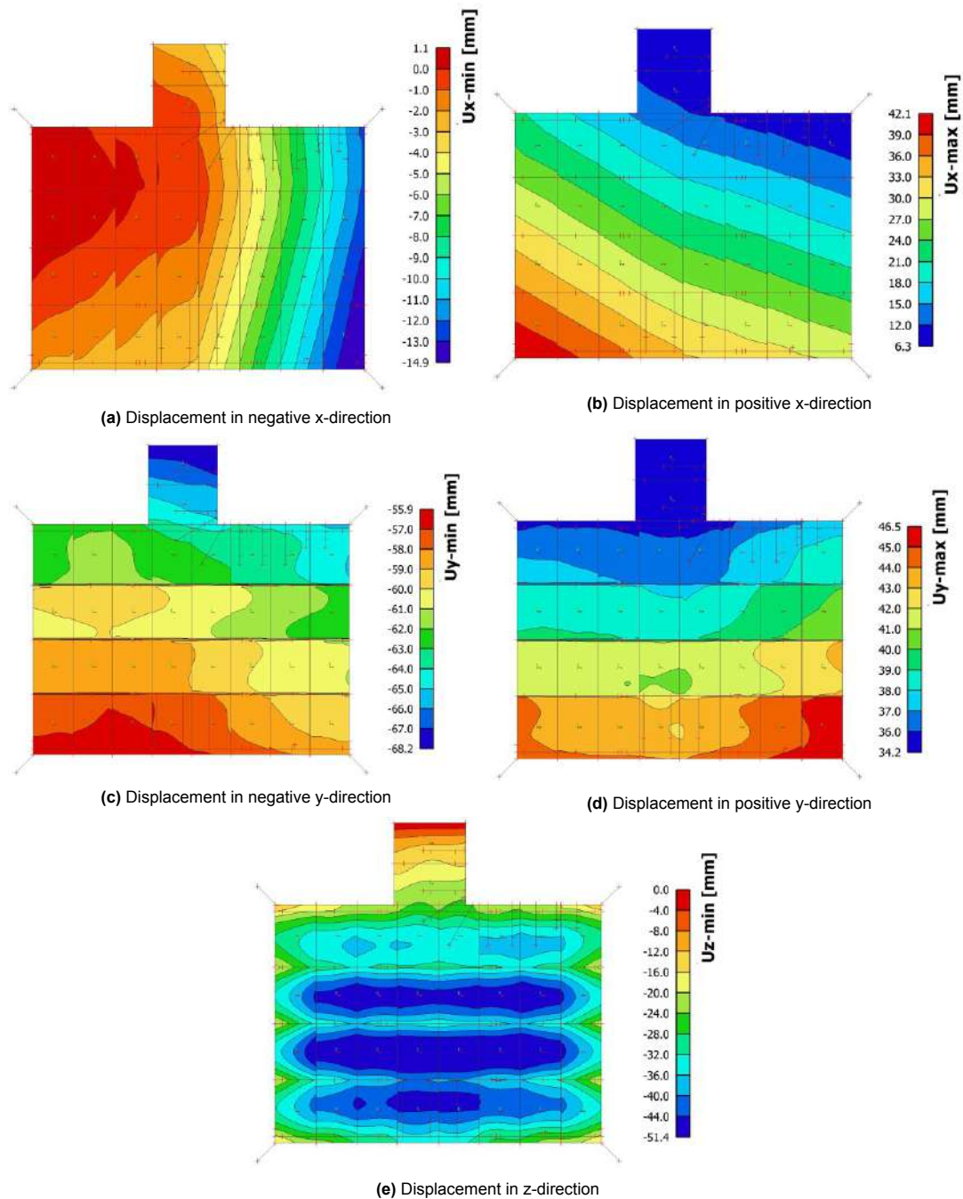
Figure E.7: Displacement of simplest solution for variant 1
