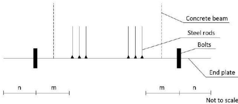
Figure E.18: Equivalent T-stub
