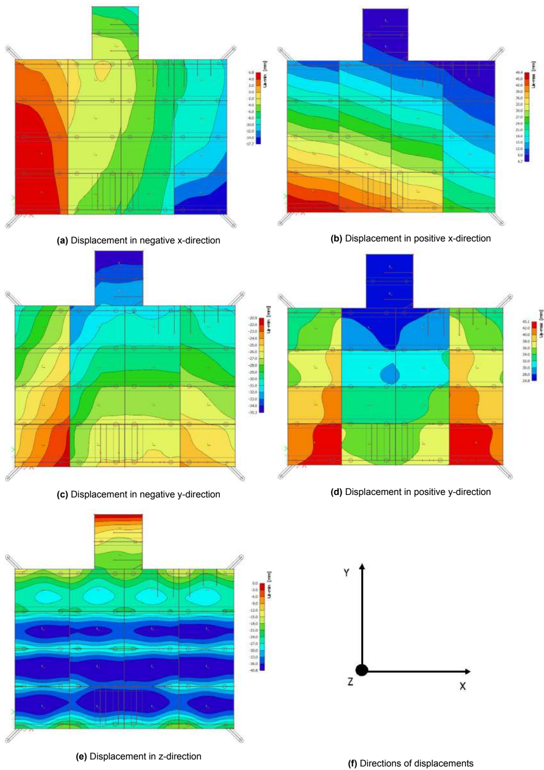
Figure 4.13: Extreme displacement of reusable jetty deck
