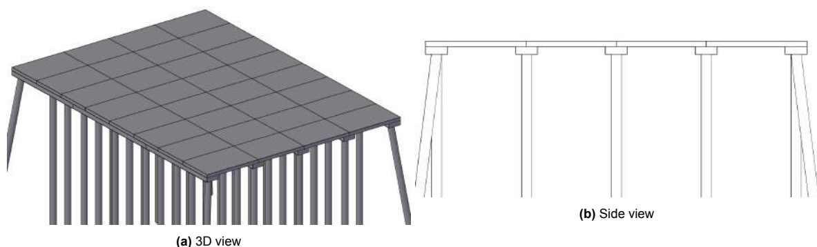
Figure E.1: Layout of variant 1: Separate rib plates and deck plates
