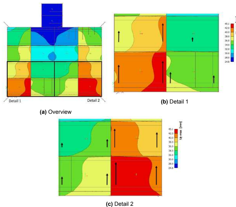
Figure 4.16: Displacement in positive y-direction of reusable jetty deck
