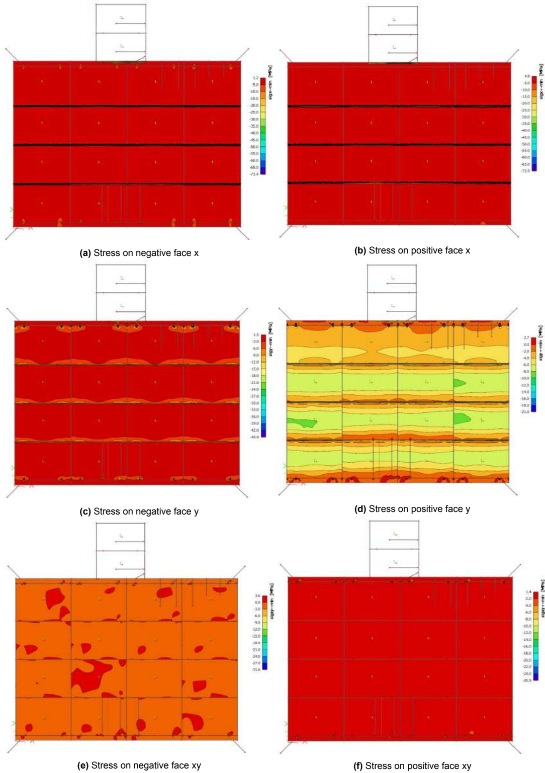
Figure 4.10: Extreme negative stresses in faces of reusable jetty deck
