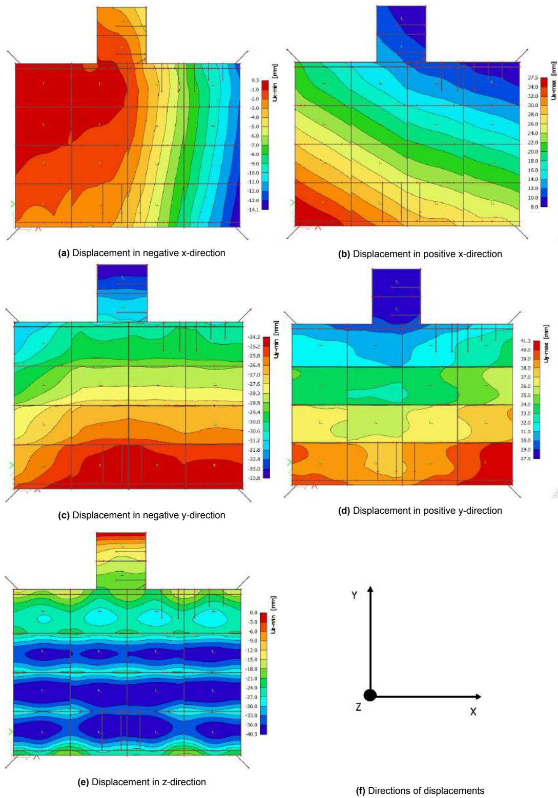
Figure 4.19: Extreme displacement of reusable jetty deck
