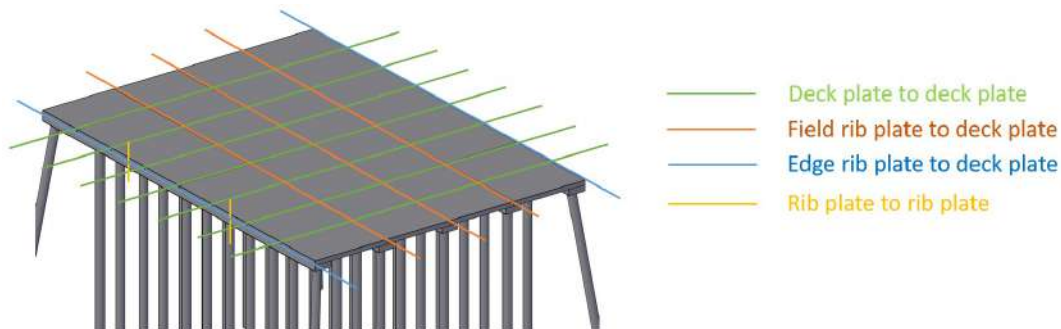
Figure E.3: Connection types in variant 1
