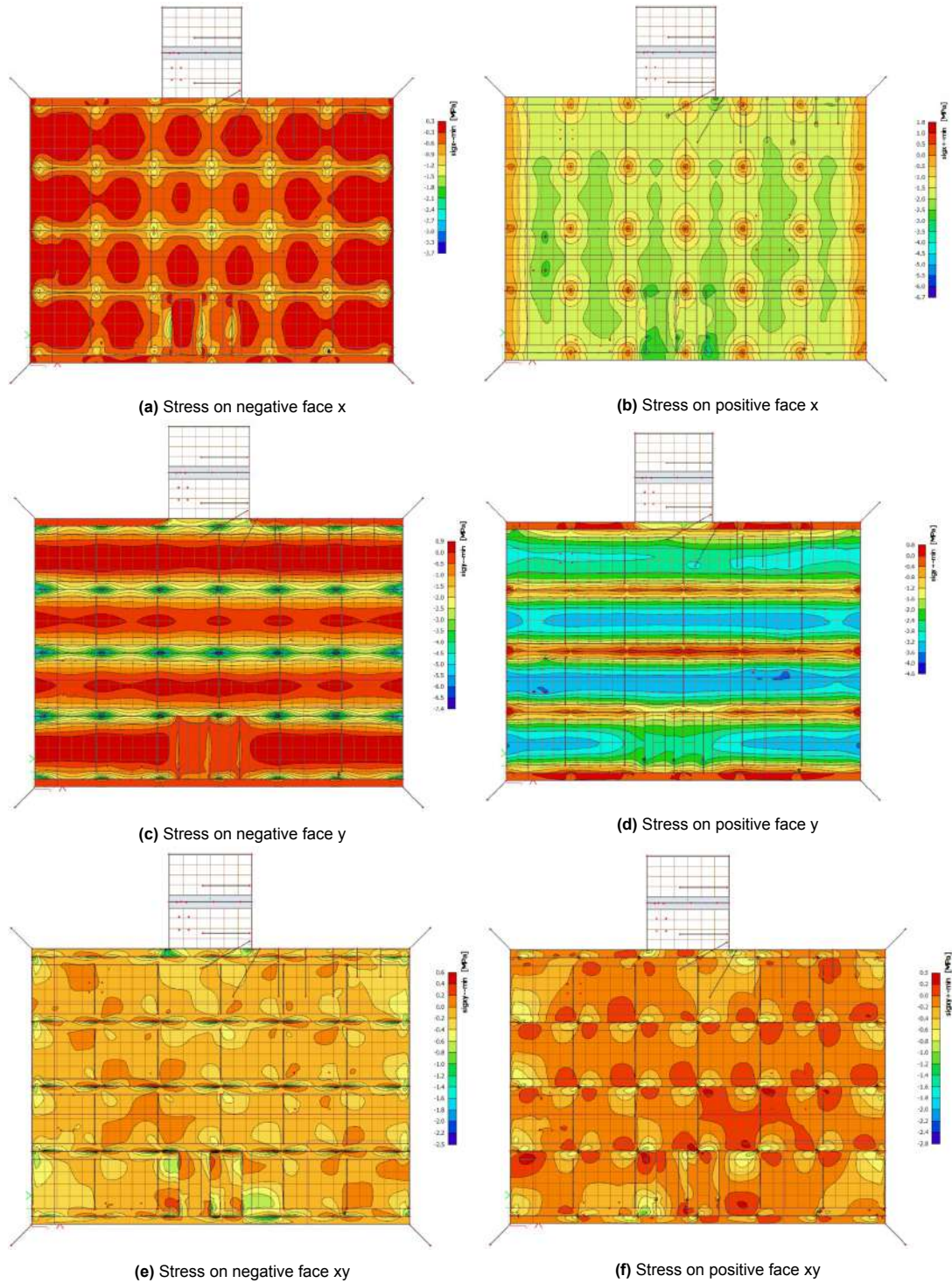
Figure 3.6: Extreme negative stresses in faces of reference jetty deck
