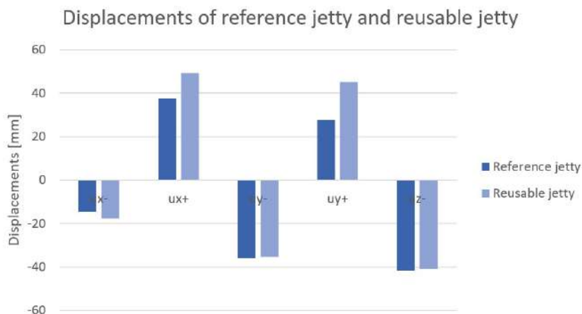
Figure 4.14: Extreme displacements of reference jetty and reusable jetty
