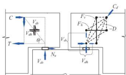
Figure 2.4: Dapped end beam connection [28]
