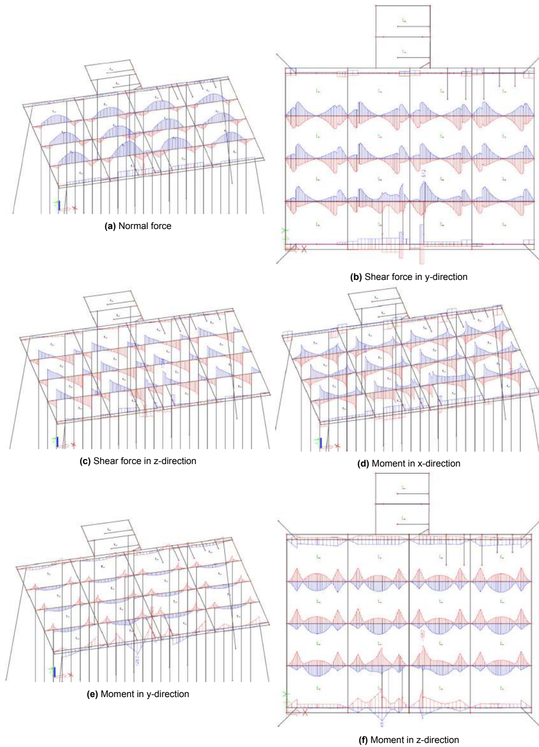
Figure 4.6: Internal forces in rib plates of reusable jetty
