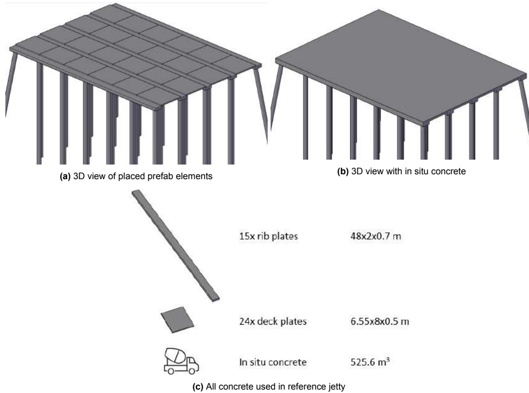
Figure 3.2: Overview of reference jetty
