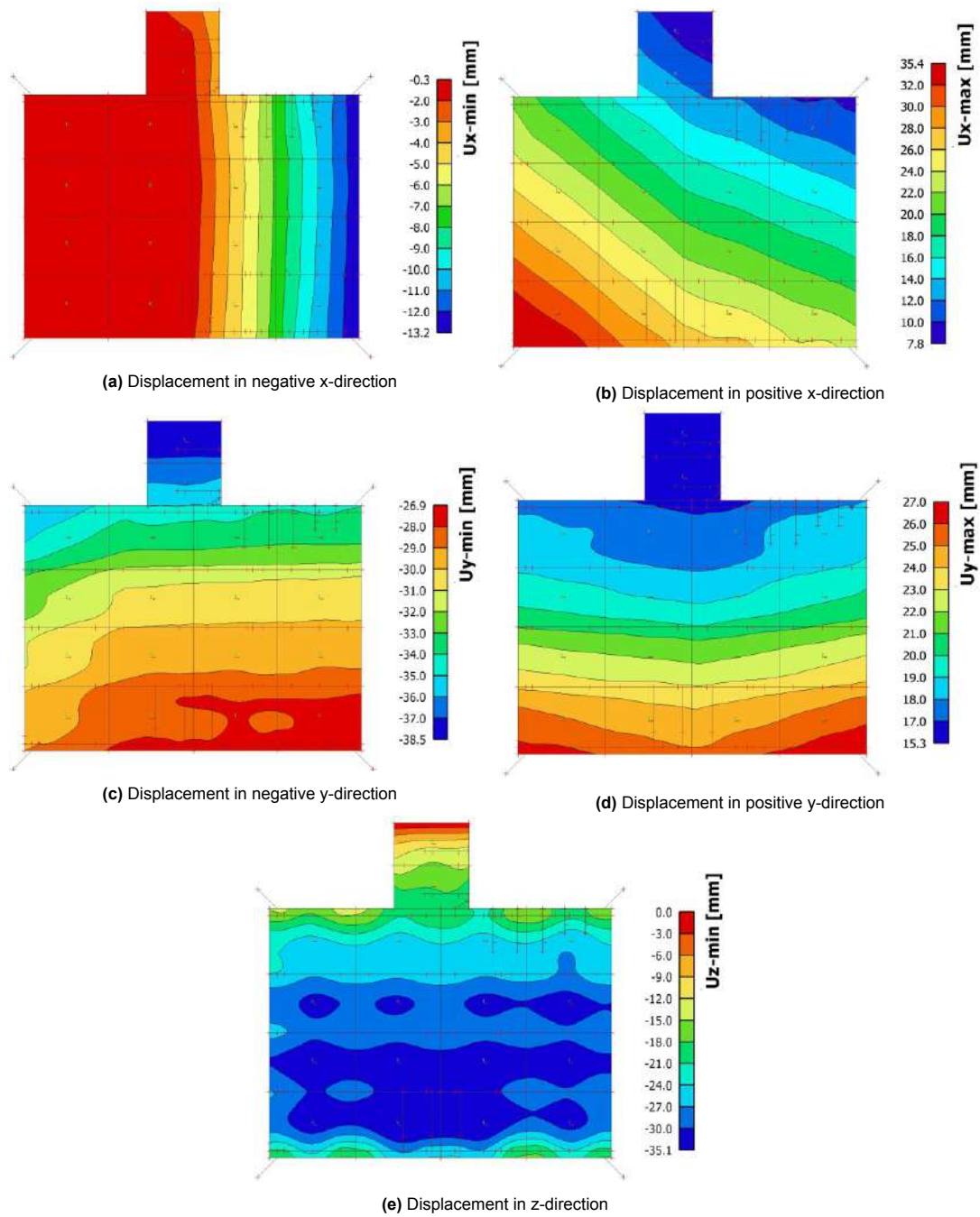
Figure F.1: Displacement of rigid solution for variant 3
