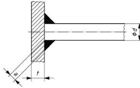
Figure E.29: Dimensions of weld [62]
