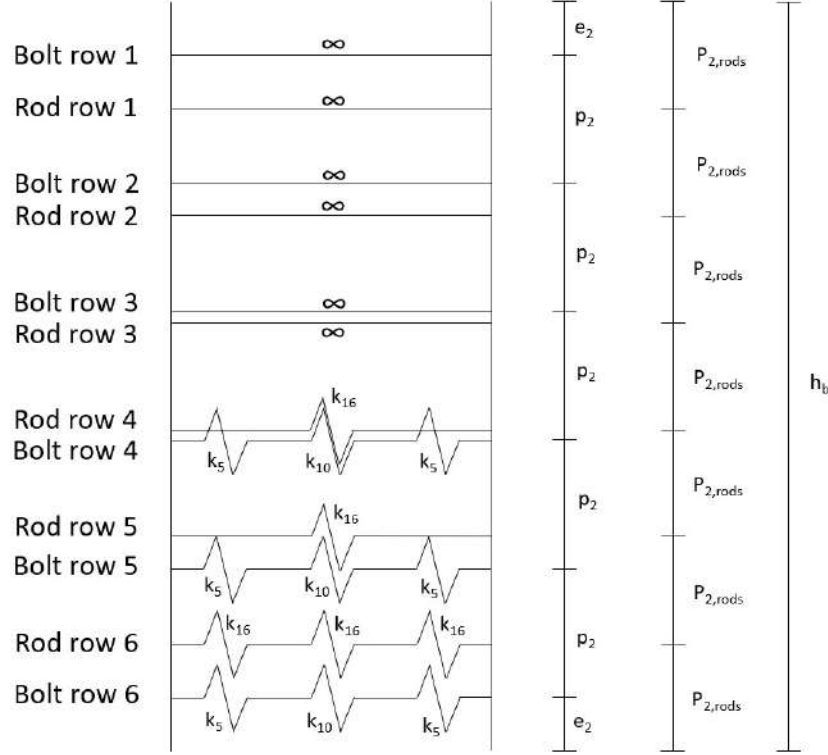
Figure E.30: Stiffness of the connection
