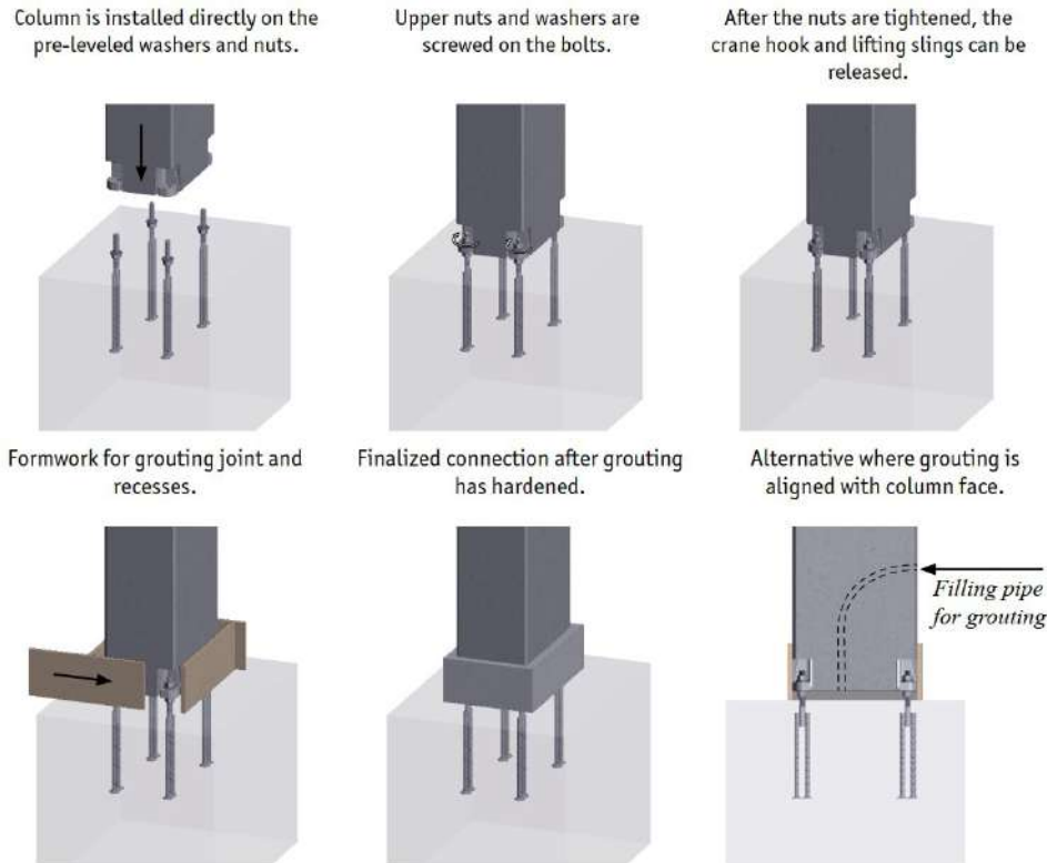
Figure E.32: Execution semi-dry connection [35]
