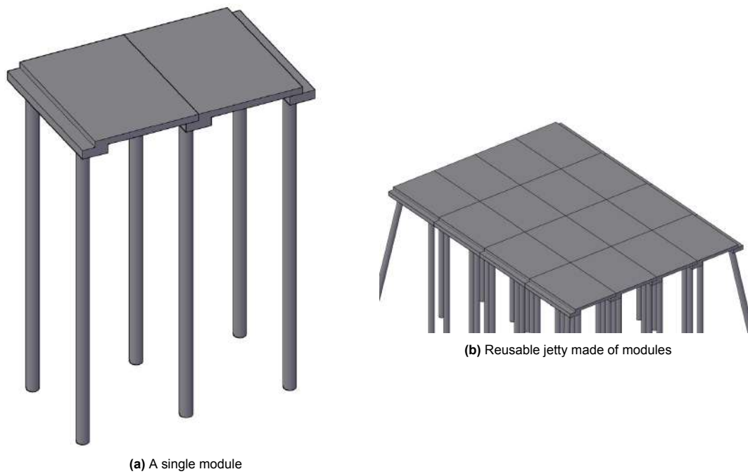
Figure 6.1: Layout of modular reusable jetty structure
