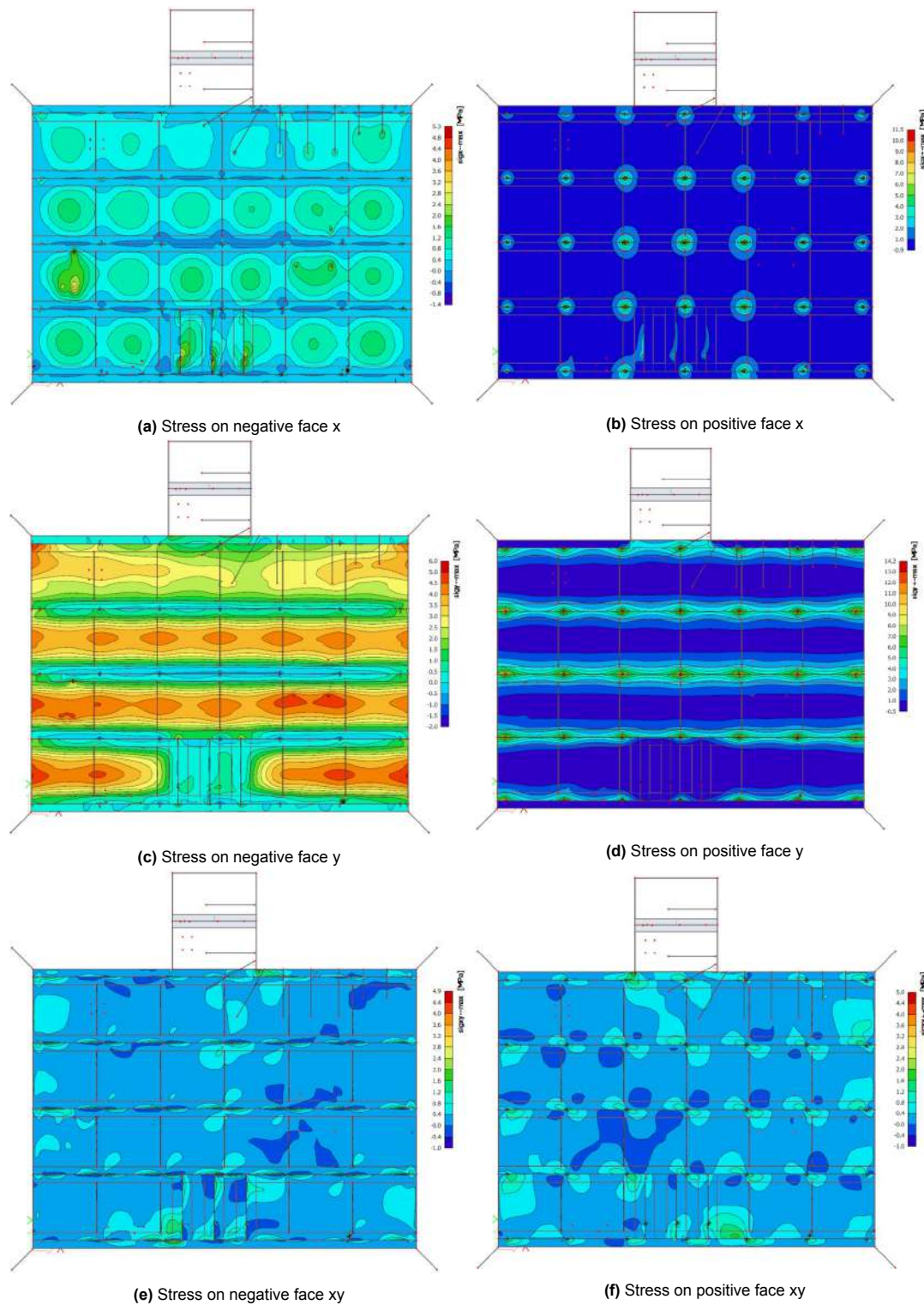
Figure 3.7: Extreme positive stress in faces of reference jetty deck
