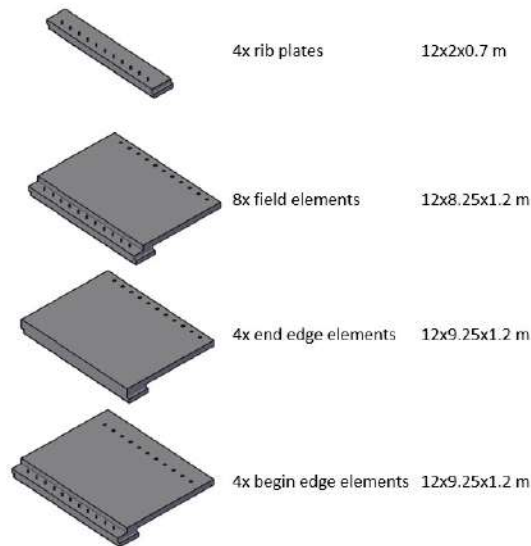
Figure 4.3: All prefab elements used in variant 3
