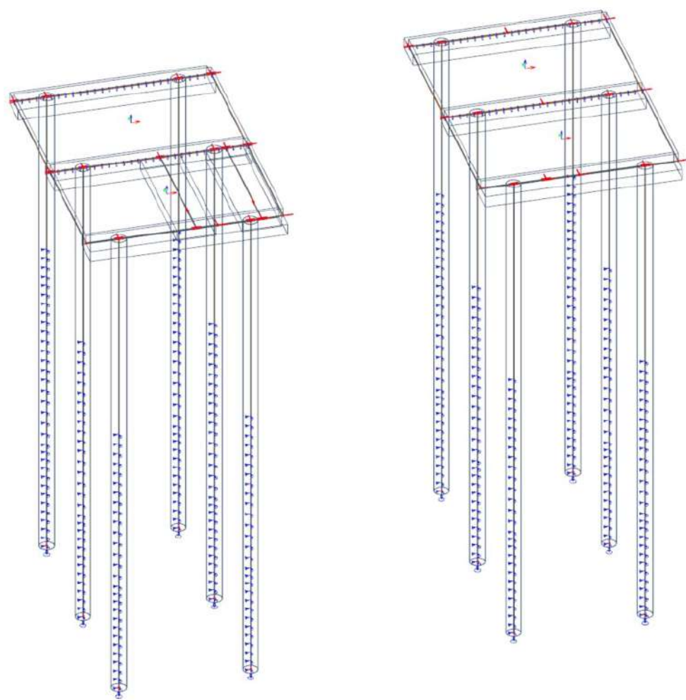
Figure D.7: Model of two separate modules
