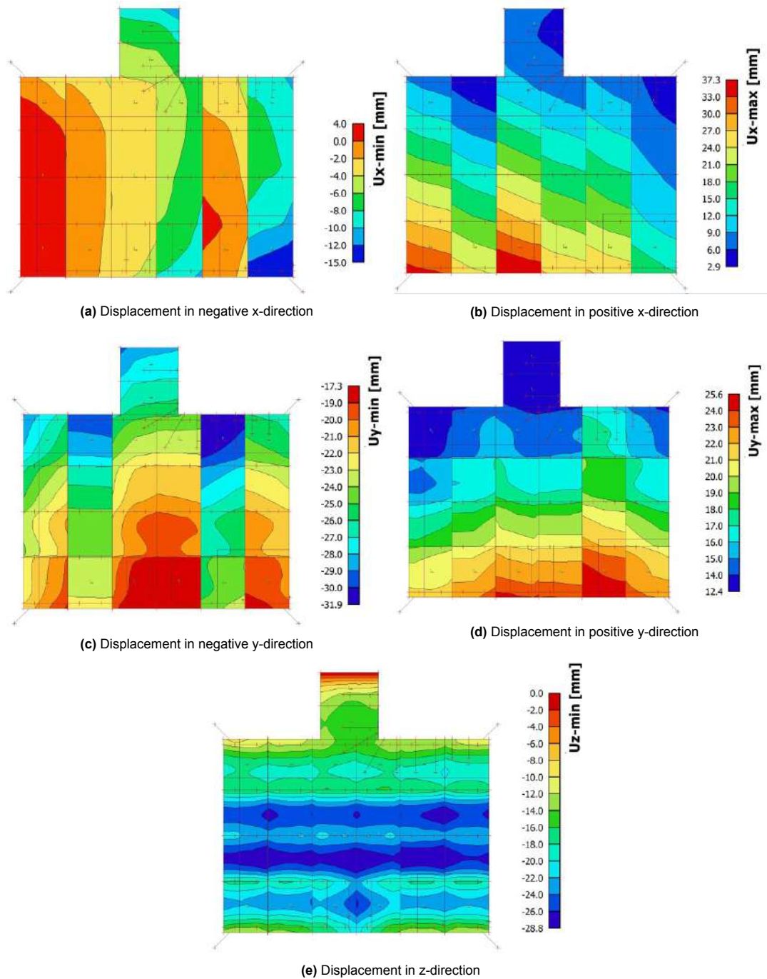
Figure E.14: Displacement of simplest solution for variant 2
