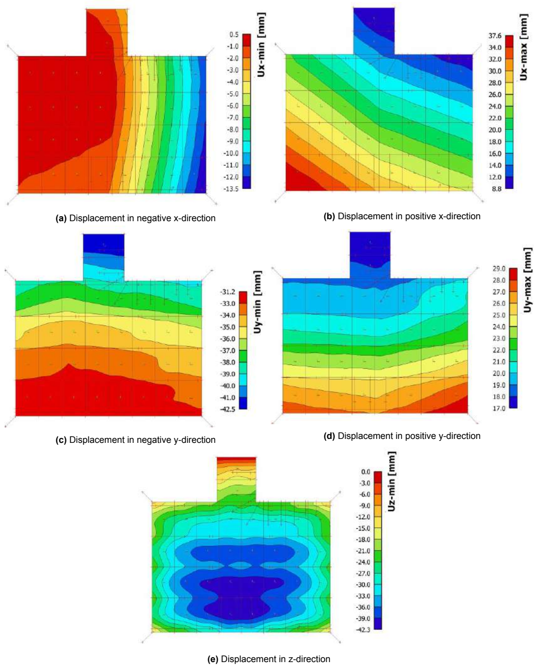
Figure E.4: Displacement of rigid solution for variant 1
