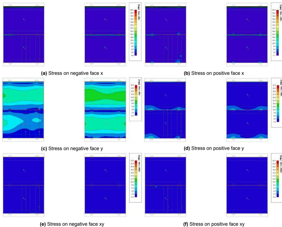
Figure F.11: Extreme positive stress in faces of modules
