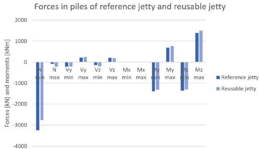
Figure 4.9: Forces in piles of reference jetty and reusable jetty
