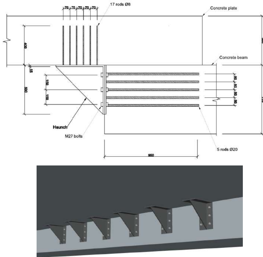
Figure E.31: Rigid beam to plate connection
