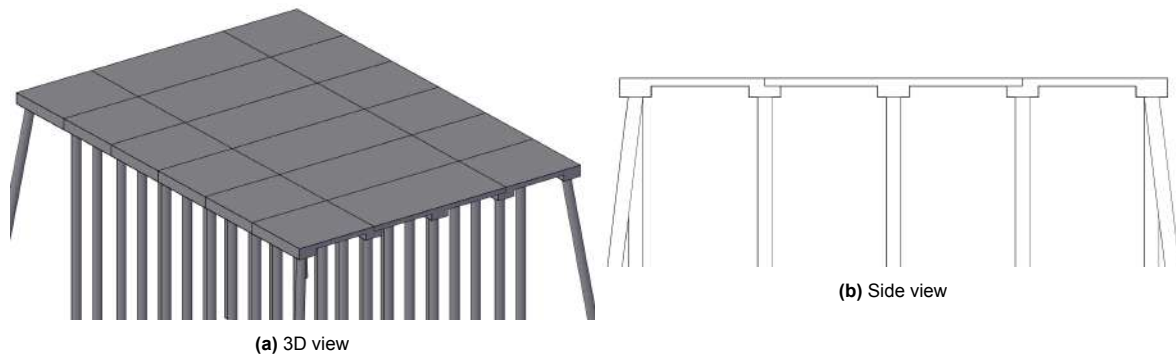
Figure E.9: Layout of variant 2: T and n-shaped elements
