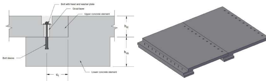
Figure 5.3: Anchor bolt concrete connection
