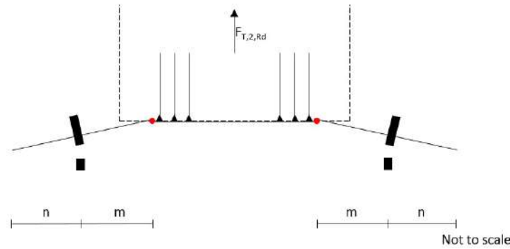
Figure E.21: Mode 2: Bolt failure with yielding of the flange
