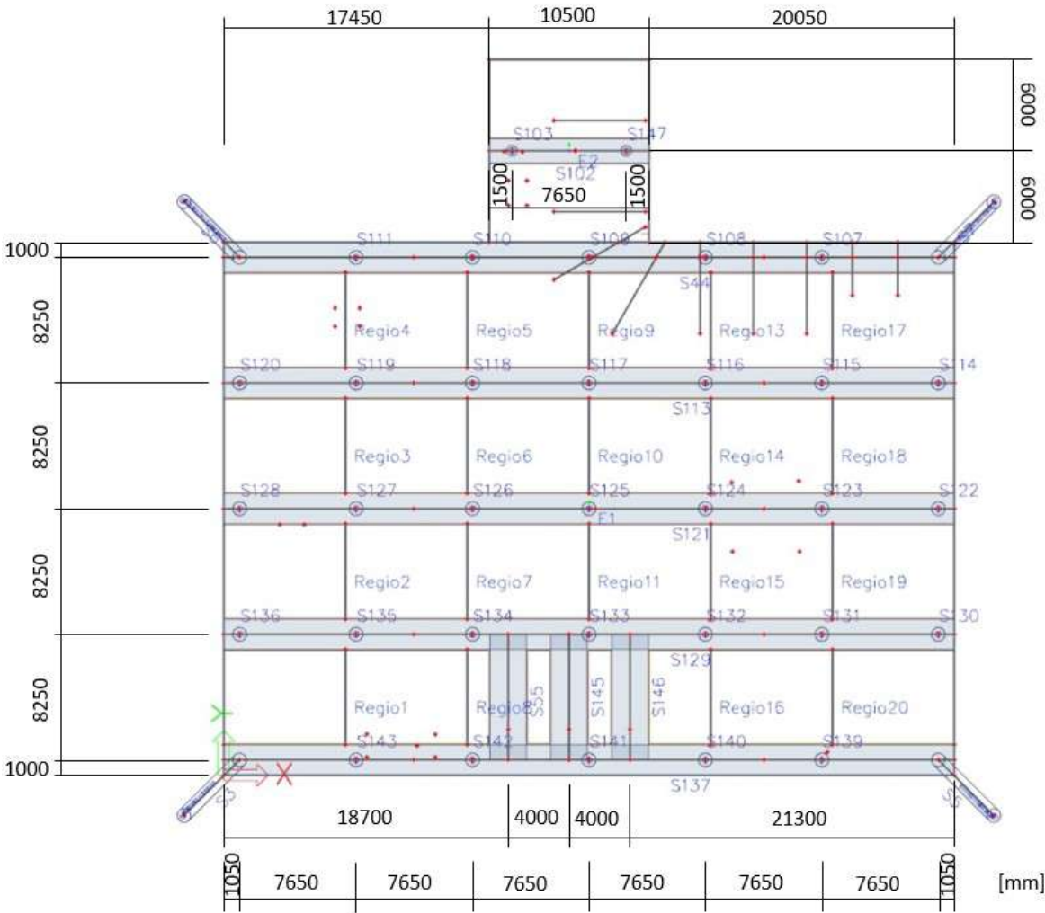
Figure D.4: Layout of reference jetty model
