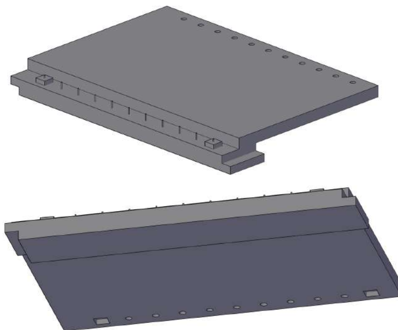
Figure 6.5: Example of element for connection with ridges and notches
