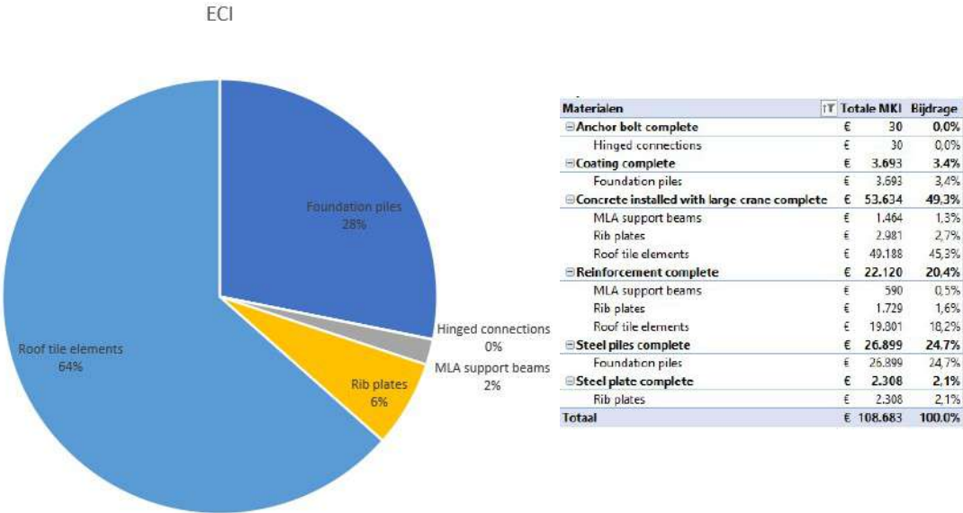
Figure G.4: Relative impact per material and element for reusable jetty
