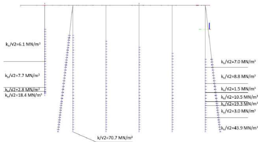
Figure 3.1: Soil modelled as springs in SCIA Engineer
