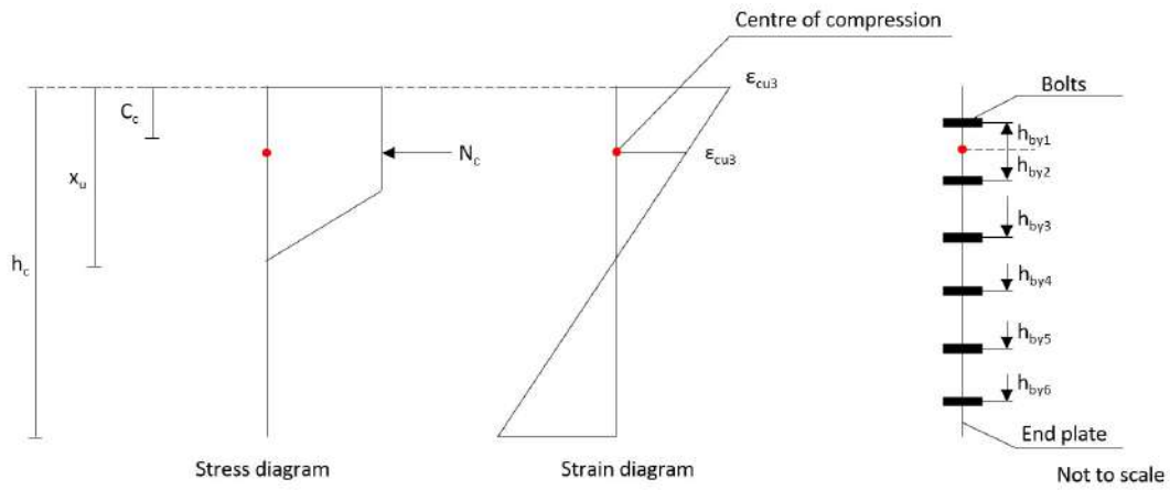
Figure E.24: Determination of centre of compression
