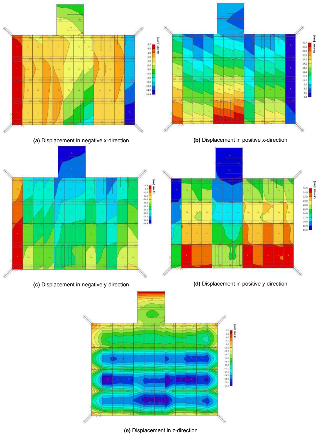
Figure F.5: Displacement of the simple solution using a regular crane for construction
