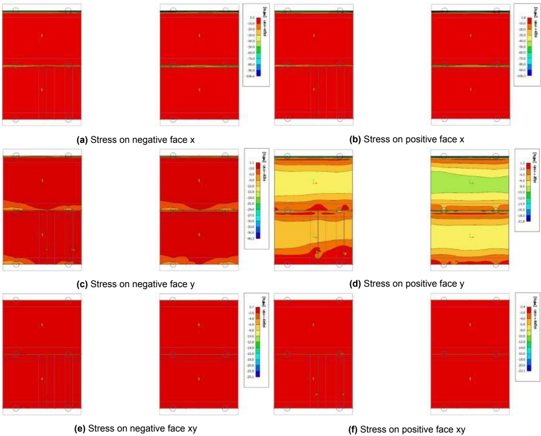
Figure F.10: Extreme negative stresses in faces of modules
