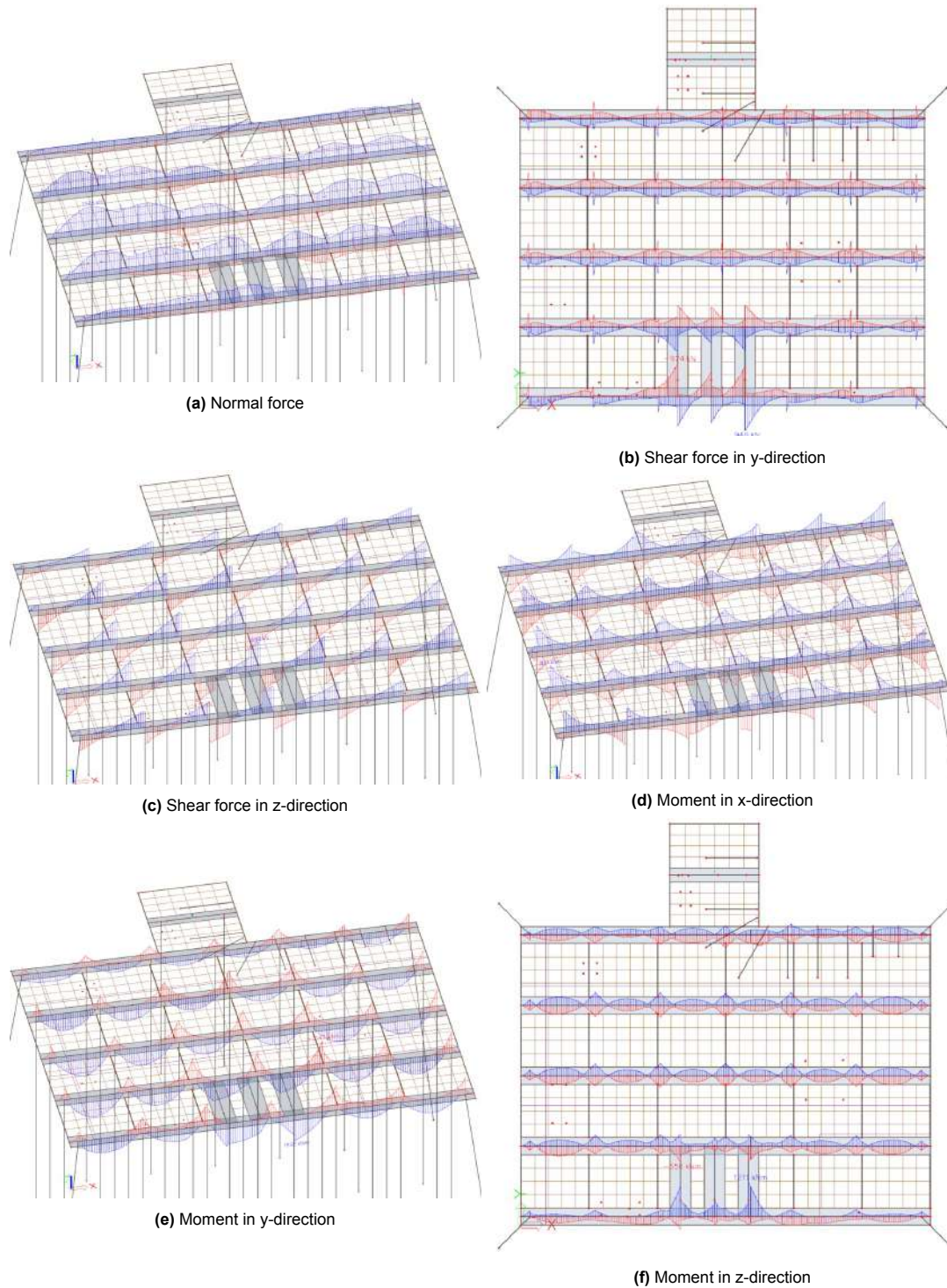
Figure 3.4: Internal forces in rib plates of reference jetty
