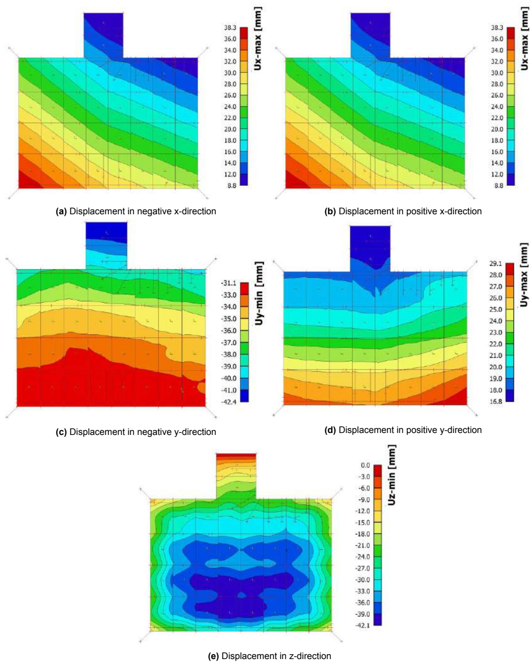
Figure E.5: Displacement with no deck plate to deck plate connection variant 1
