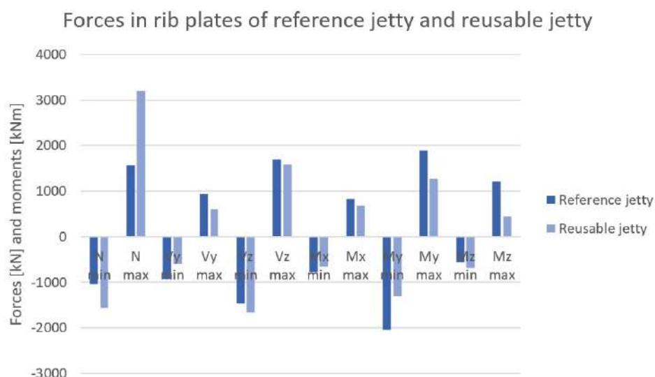
Figure 4.7: Forces in rib plates of reference jetty and reusable jetty
