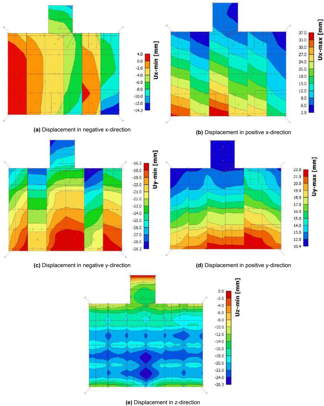
Figure E.13: Displacement of no plate-part to plate-part and shear rib plate to rib plate connection variant 2
