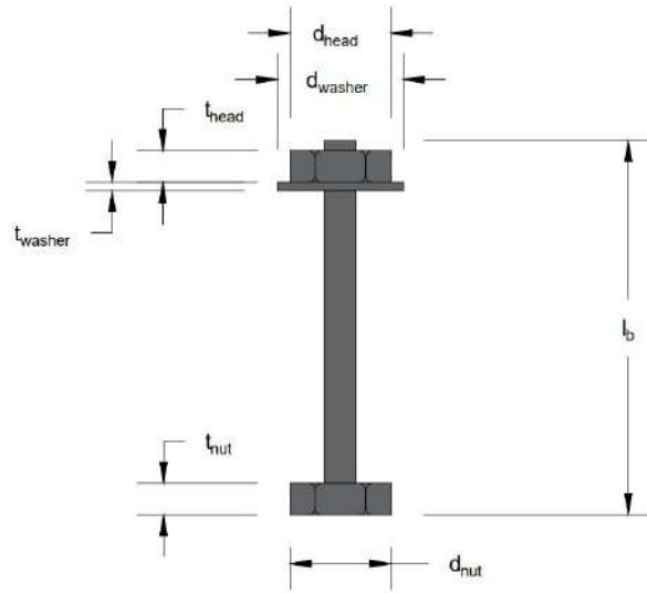
Figure F.6: Dimensions of the anchor bolt
