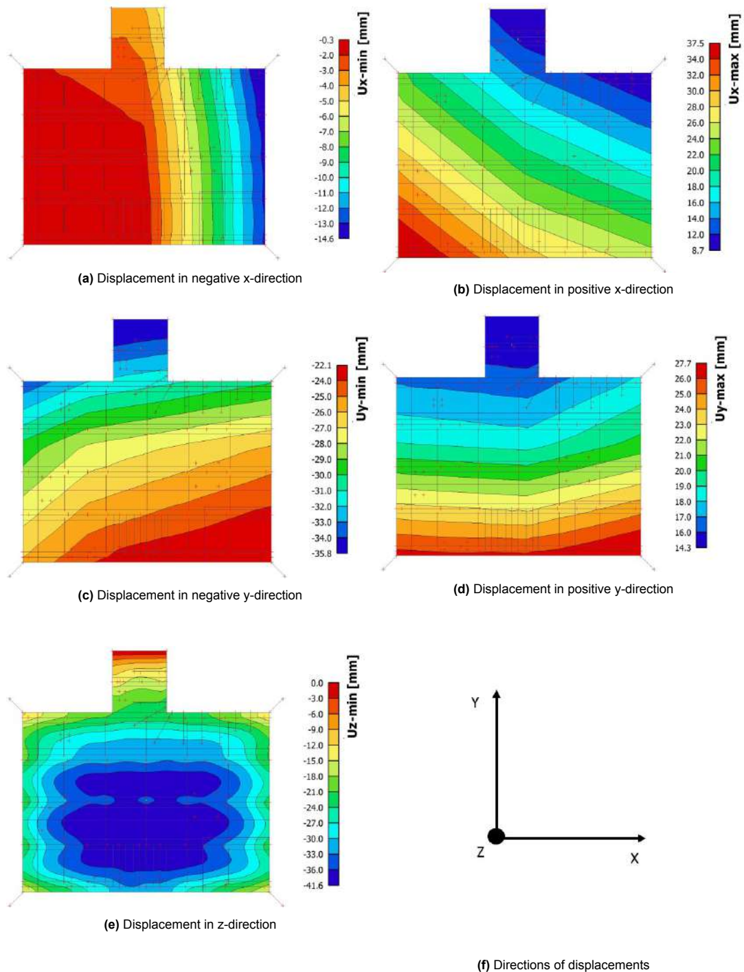
Figure 3.8: Extreme displacement of reference jetty deck
