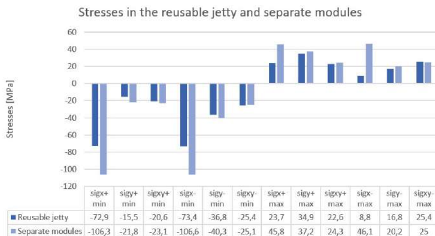
Figure 6.4: Comparison of stresses in reusable jetty and separate modules
