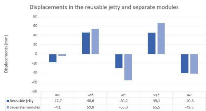
Figure 6.3: Comparison of displacements in reusable jetty and separate modules
