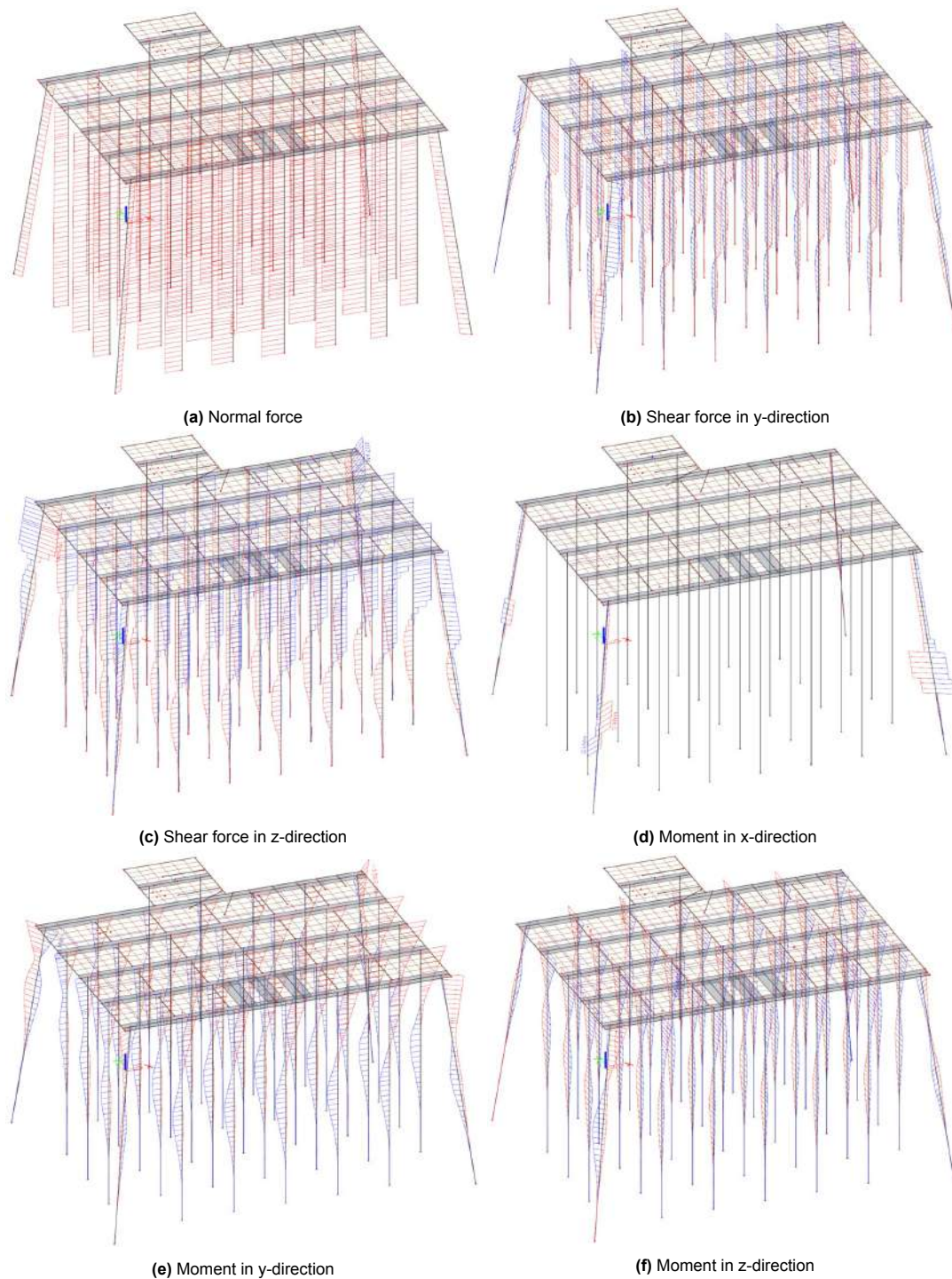
Figure 3.5: Internal forces in piles of reference jetty
