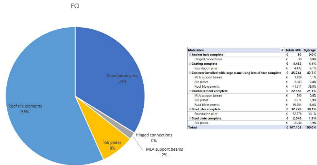
Figure G.12: Relative impact per material and element for modular reusable jetty with low clinker concrete
