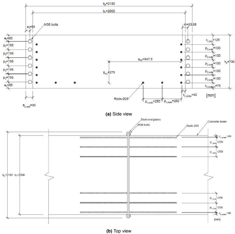
Figure E.17: Layout of rigid rib plate to rib plate connection
