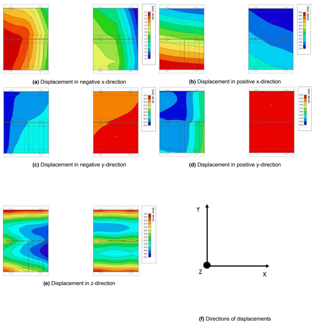
Figure 6.2: Displacement of reusable jetty modules
