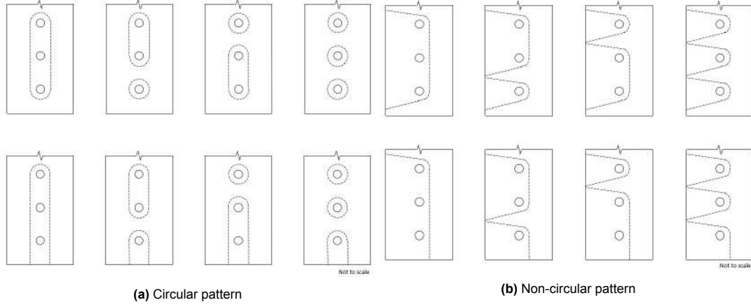
Figure E.19: Effective lengths for bolts in tension
