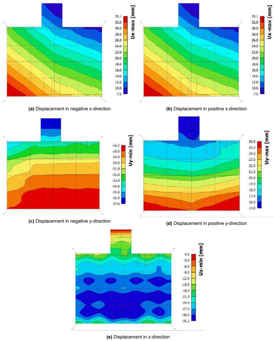
Figure F.2: Displacement with no deck plate to deck plate connection variant 3
