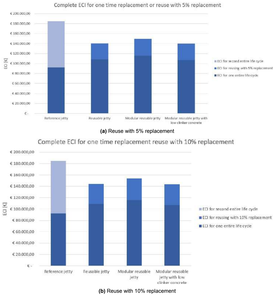
Figure 7.2: ECI comparison for one time reuse
