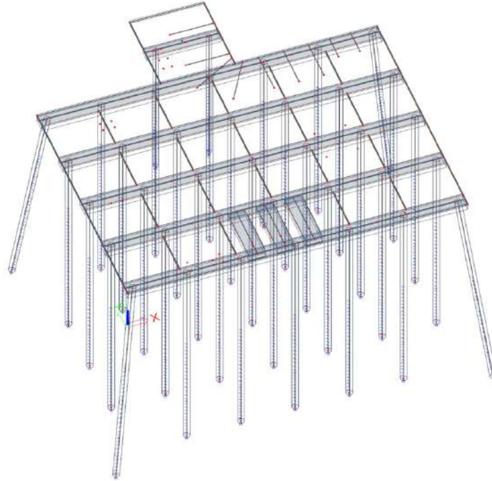
Figure 3.3: Overview of model reference jetty
