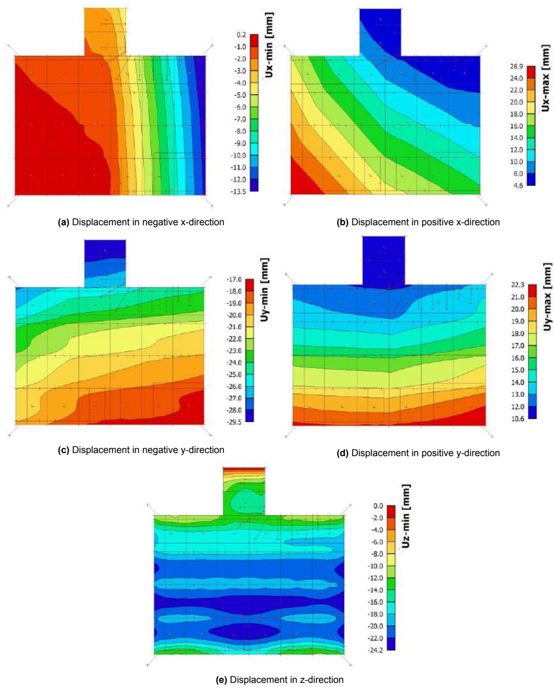
Figure E.12: Displacement of rigid solution for variant 2
