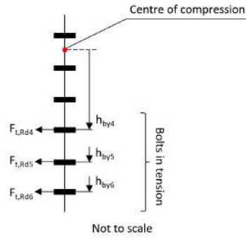
Figure E.23: Bending moment resistance of connection
