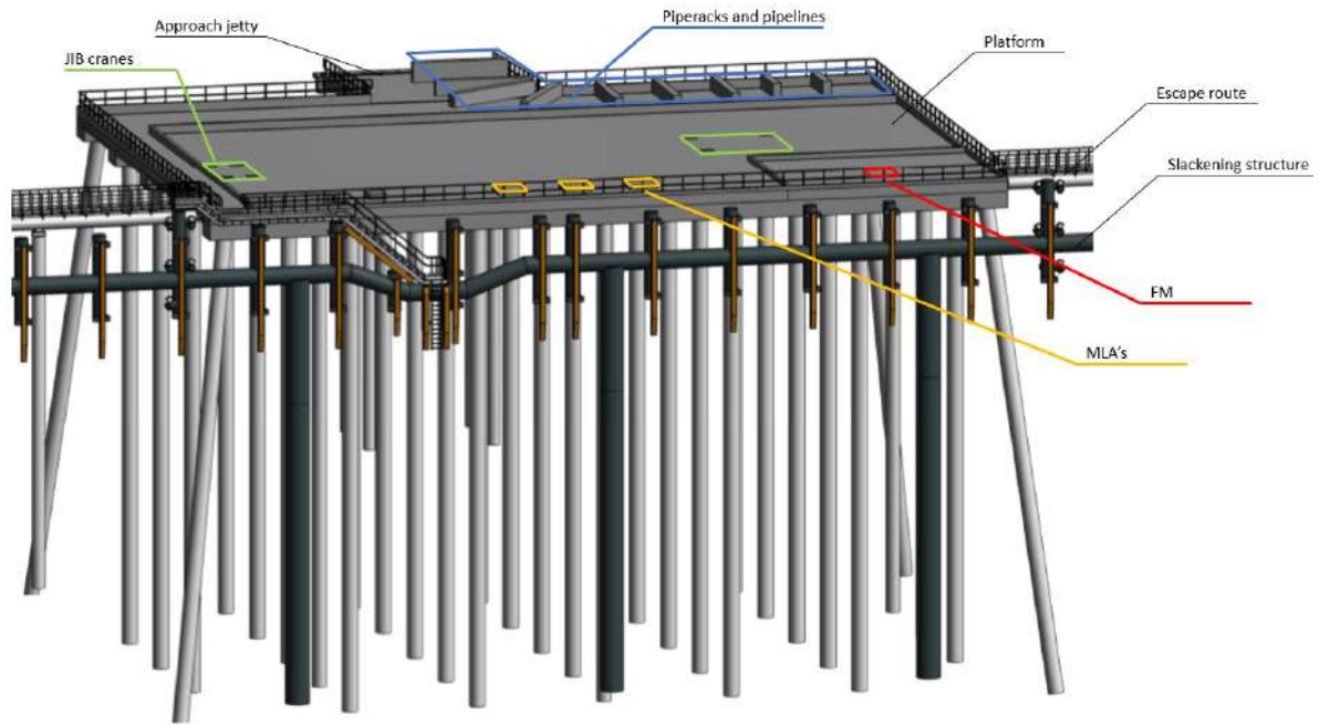
Figure C.2: Overview of reference jetty parts, MLA's, piperacks and pipelines
