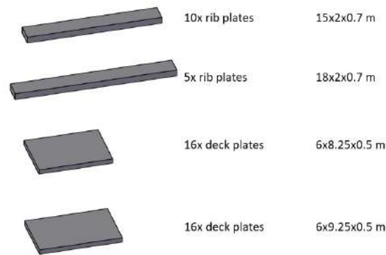
Figure E.2: All prefab elements used in variant 1
